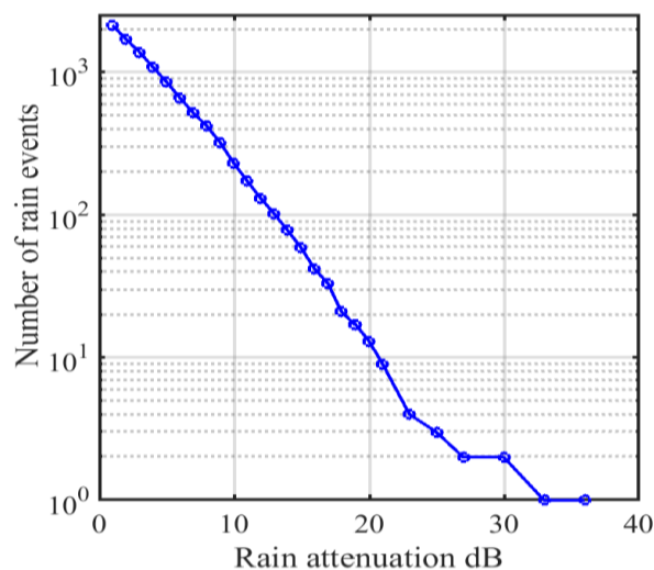
FIGURE 10. Total number of fading events for a given fade amplitude
