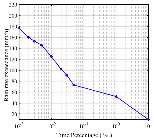
FIGURE 4. Cumulative distribution of the one-year measured rain rate
