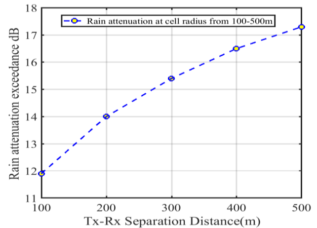
FIGURE 9. Predicted rain attenuation versus path length at cell radius from 100-500 meters using [62]
