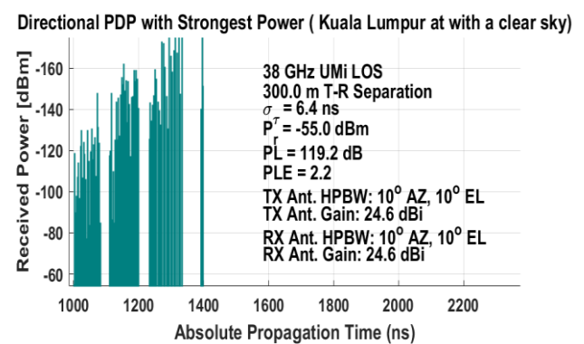
FIGURE 12. Directional PDP at clear sky status
