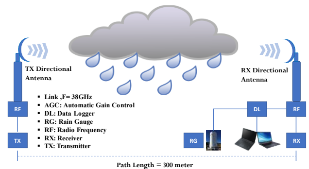
FIGURE 3. The block diagram of the measurement equipment for data collection of rain rate and rain attenuation
