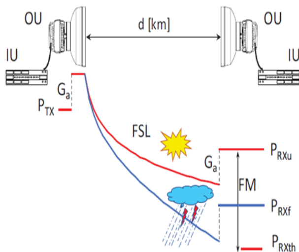
FIGURE 1. Link budget and fade margin calculation source [49]
