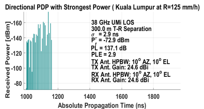
FIGURE 13. Directional PDP at heavy rain status
