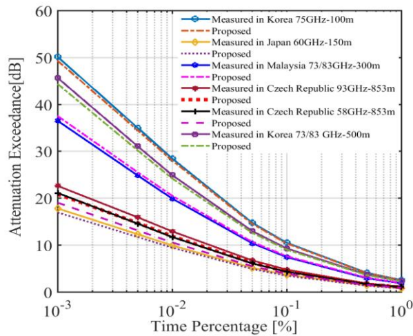
FIGURE 8. Measured and predicted rain attenuation using the proposed model in [51] at F > 40 GHz and path length < 1 km
