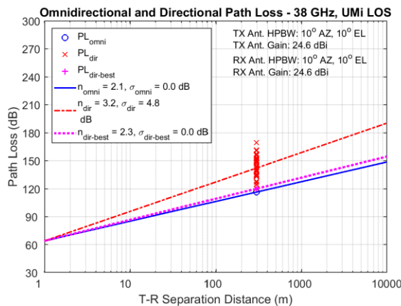
FIGURE 16. CI path loss model at 38 GHz for outdoor D2D link with 28°C sunny sky (htx=17.3, hrx=1.5 m)
