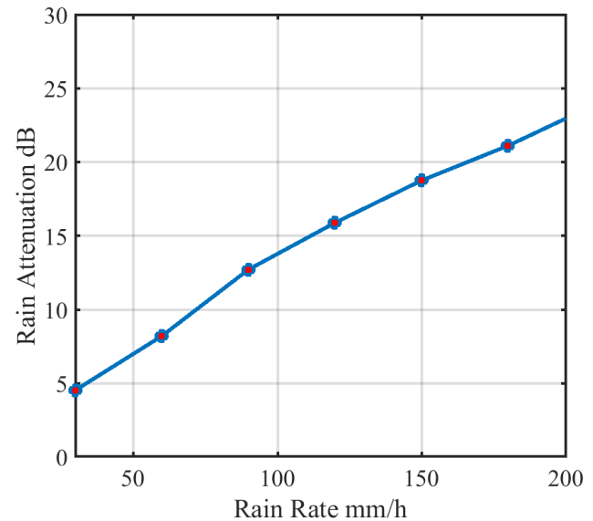
FIGURE 6. Cumulative distribution of measured rain rate of one year versus rain attenuation at 38 GHz over 300 m
