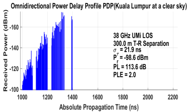
FIGURE 14. Omnidirectional PDP at clear sky status
