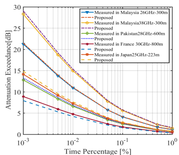
FIGURE 7. Measured and predicted rain attenuation using the proposed model in [51] at F < 40 GHz and path length < 1 km
