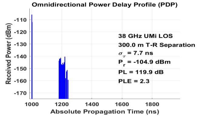
FIGURE 15. Omnidirectional PDP at heavy rain status
