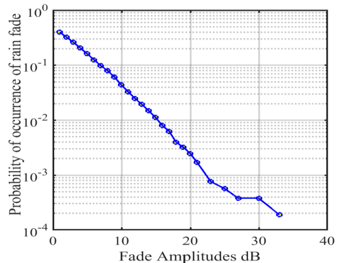
FIGURE 11. Probability of rain attenuation occurrences for different measured attenuation levels at 38 GHz and 300 m path length
