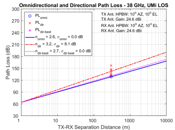
FIGURE 17. CI path loss model at 38 GHz for outdoor D2D link with a rain rate of 125 mm/h (htx=17.3, hrx=1.5 m)
