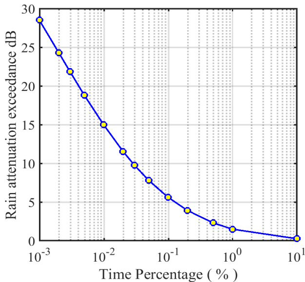
FIGURE 5. Cumulative distribution for the maximum rain attenuation at 300 m link
