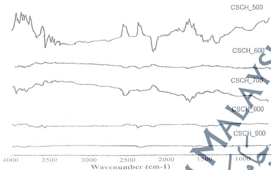
Figure 2.6 FTIR spectra of cocoa shell-based activated carbons at different carbonization temperatures (Ahmad et al., 2013a).
