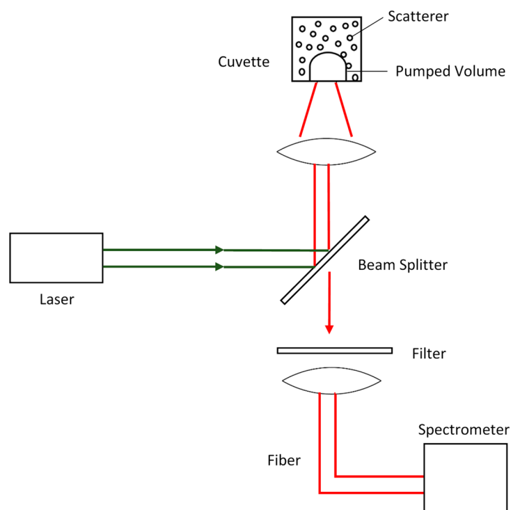
Figure 1. Optical layout of random lasers.
