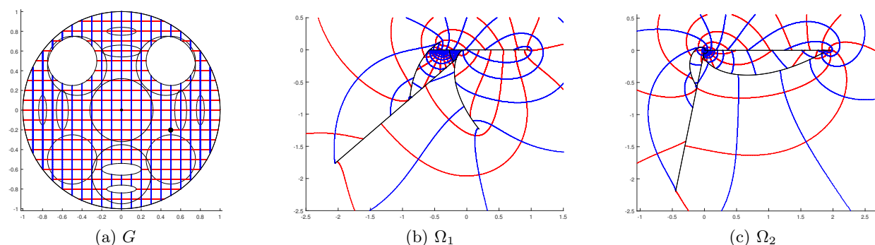
Figure 2: The original image G and its image \Omega_1 (center) \Omega_2 (right) for Example 1.
