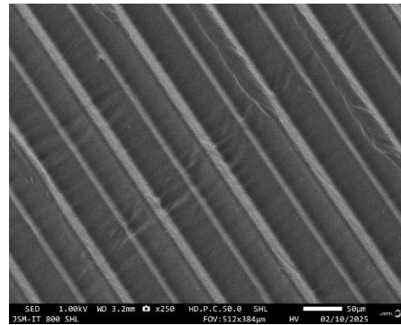
Figure 2: Surface microscopy of 3D_DLP
