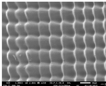
Figure 3: Surface microscopy of 3D_SLA
