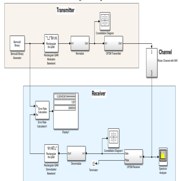
Fig. 1. OFDM system 64-QAM in a noisy Multipath Rician Channel
