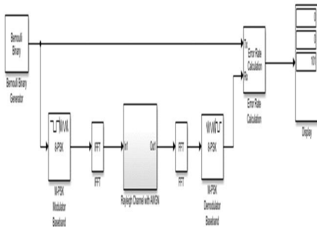
Fig. 2. OFDM based system using BPSK Modulation
