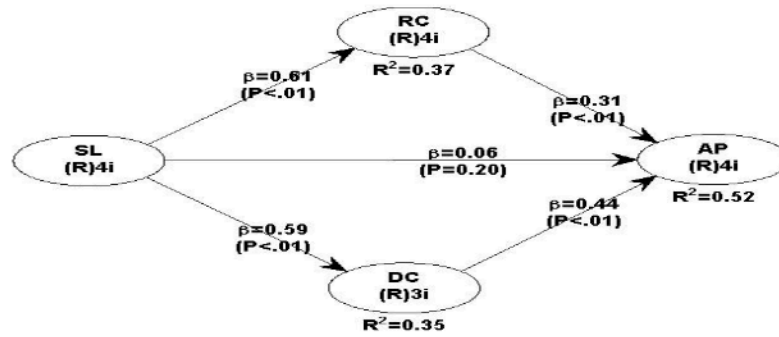
Figure 1. Path Diagram of the Structural Model in PLS
