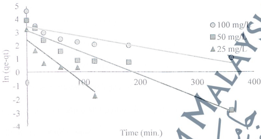
Figure 6.9 Pseudo-first-order kinetic model of paracetamol adsorption.
